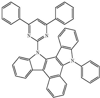
[Chemical formula 18]
