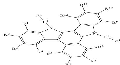
[Chemical formula 1]
