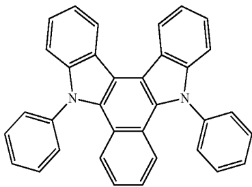
[Chemical formula 18]
